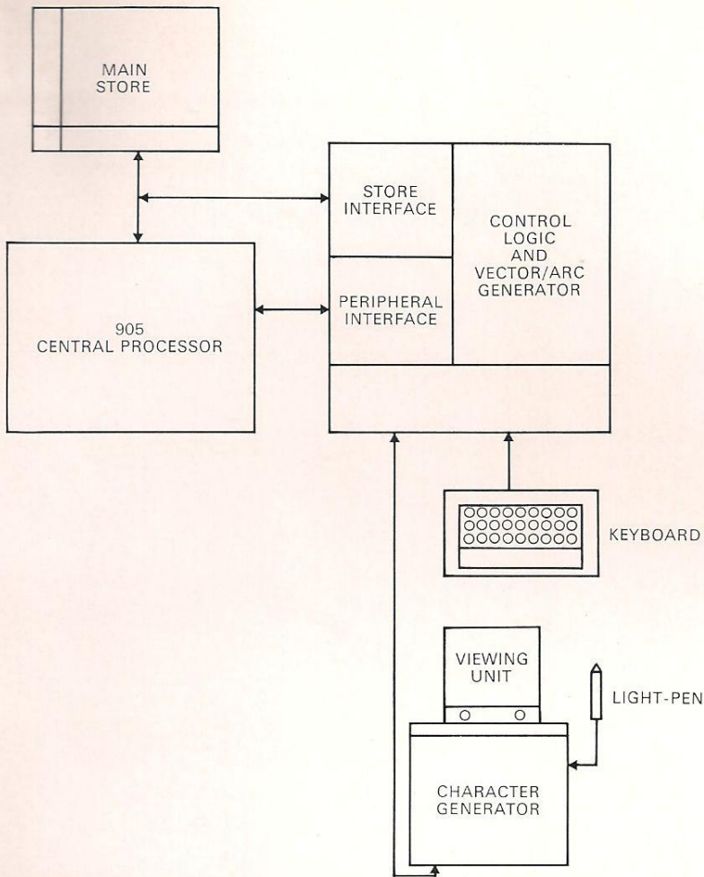
928 Display System block diagram
